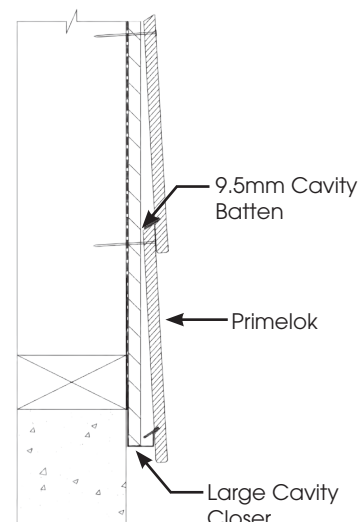
9.5mm Cavity Batten Primelok
