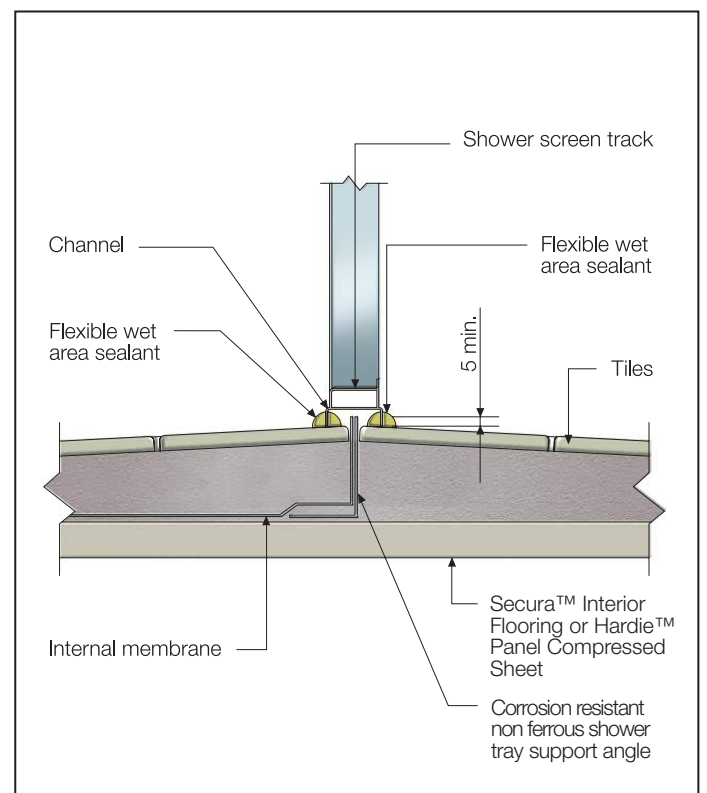
FIGURE 19 HOBLESS SHOWER
