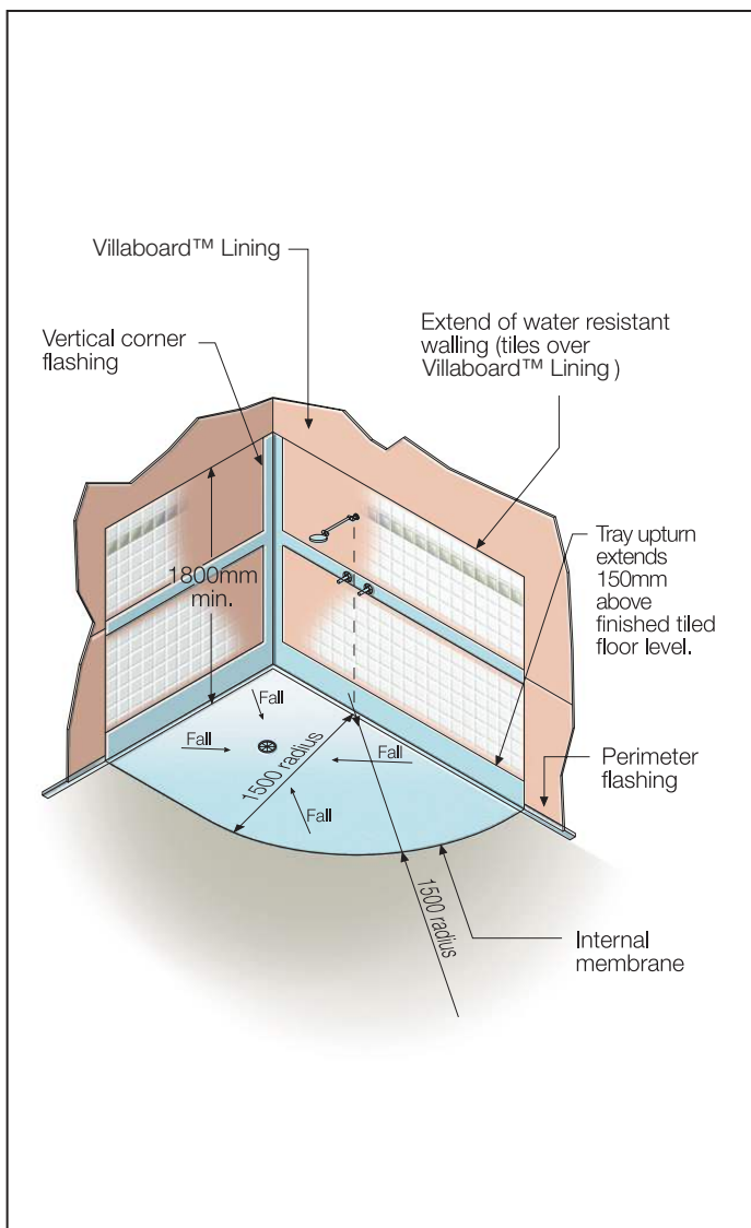
FIGURE 20 UNENCLOSED SHOWERS
