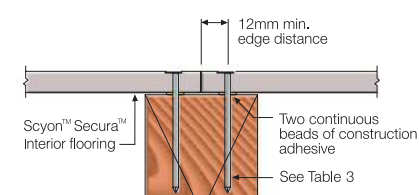
FIGURE 5 FIXING 2ND PANEL
