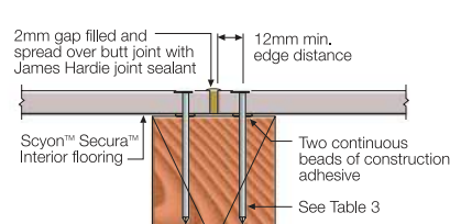
FIGURE 6 BUTT JOINING OPTIONS
