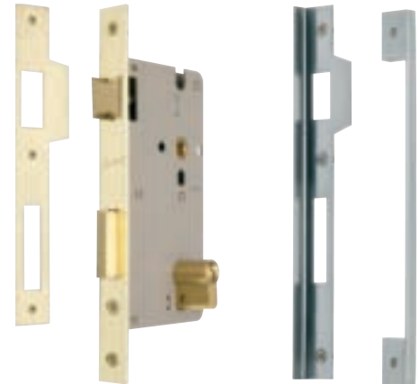
755 Mortice Lock Double Cylinder SC
